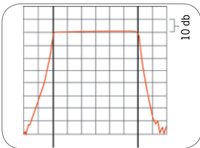
ZF150 Frequency Response
